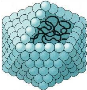
Mastadenavirus
